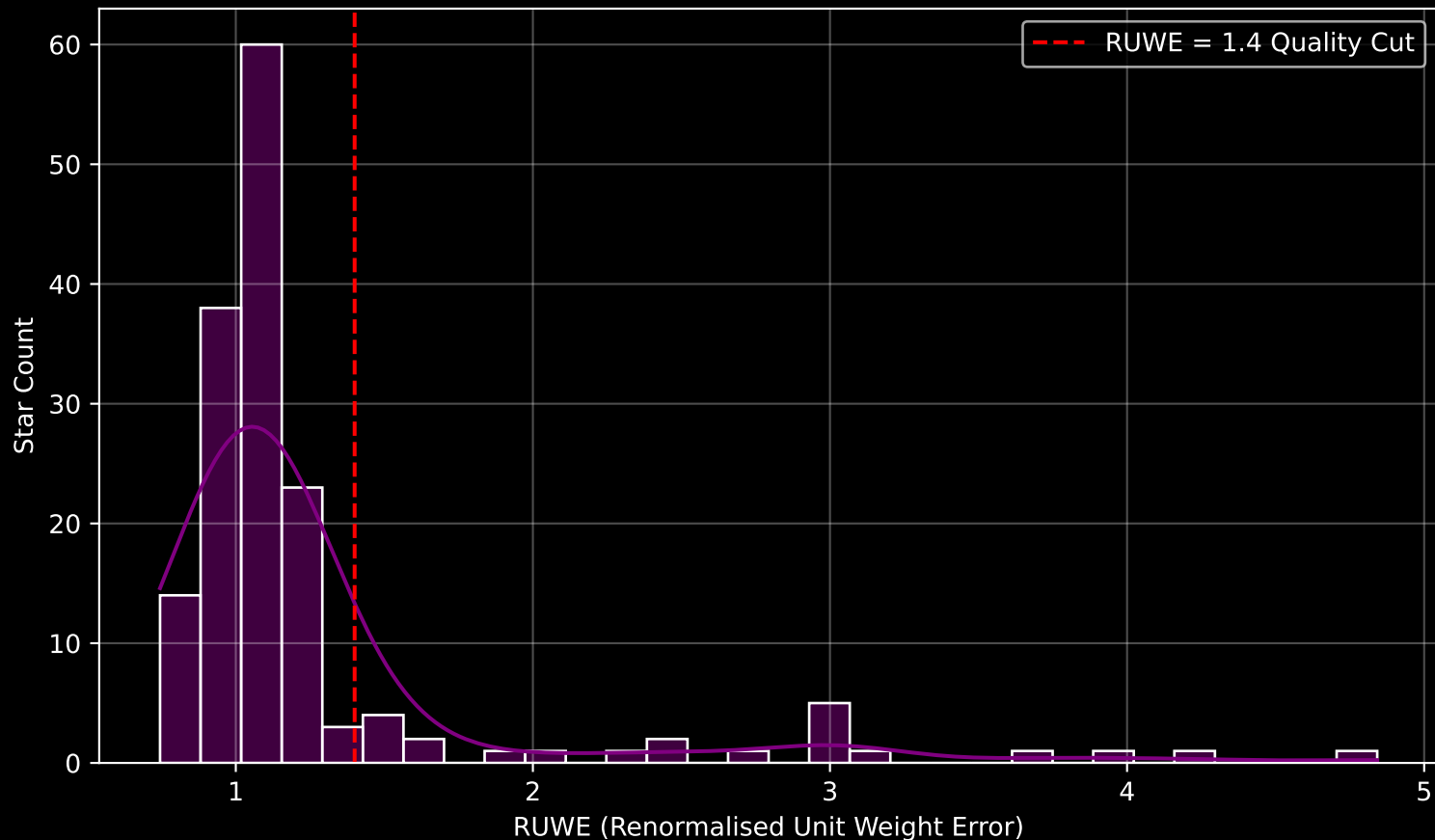
GAPOGEE DR17 Field [279-24-O_TESS] RUWE Distribution (n= 160)
