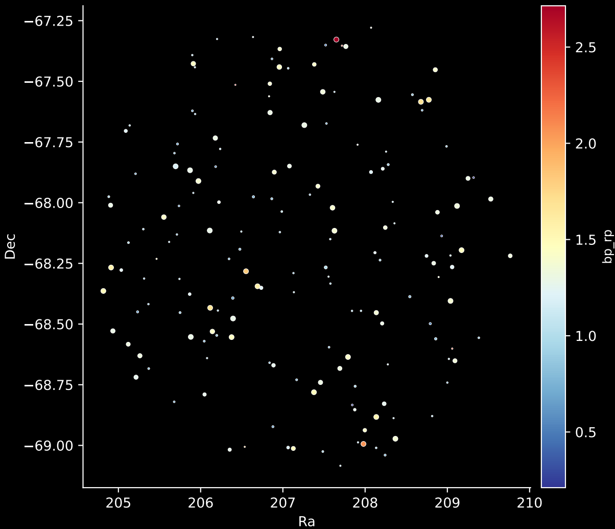
APOGEE DR17 Field: [279-24-O_TESS] Stars: 168
