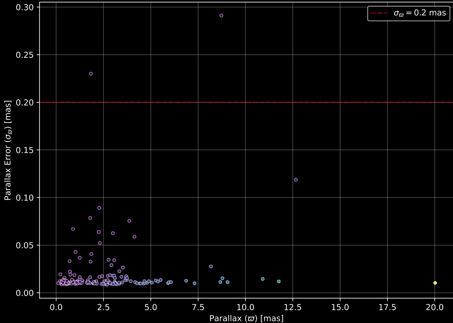
APOGEE DR17 Field: [279-24-O_TESS] Parallax Quality (n= 168)
