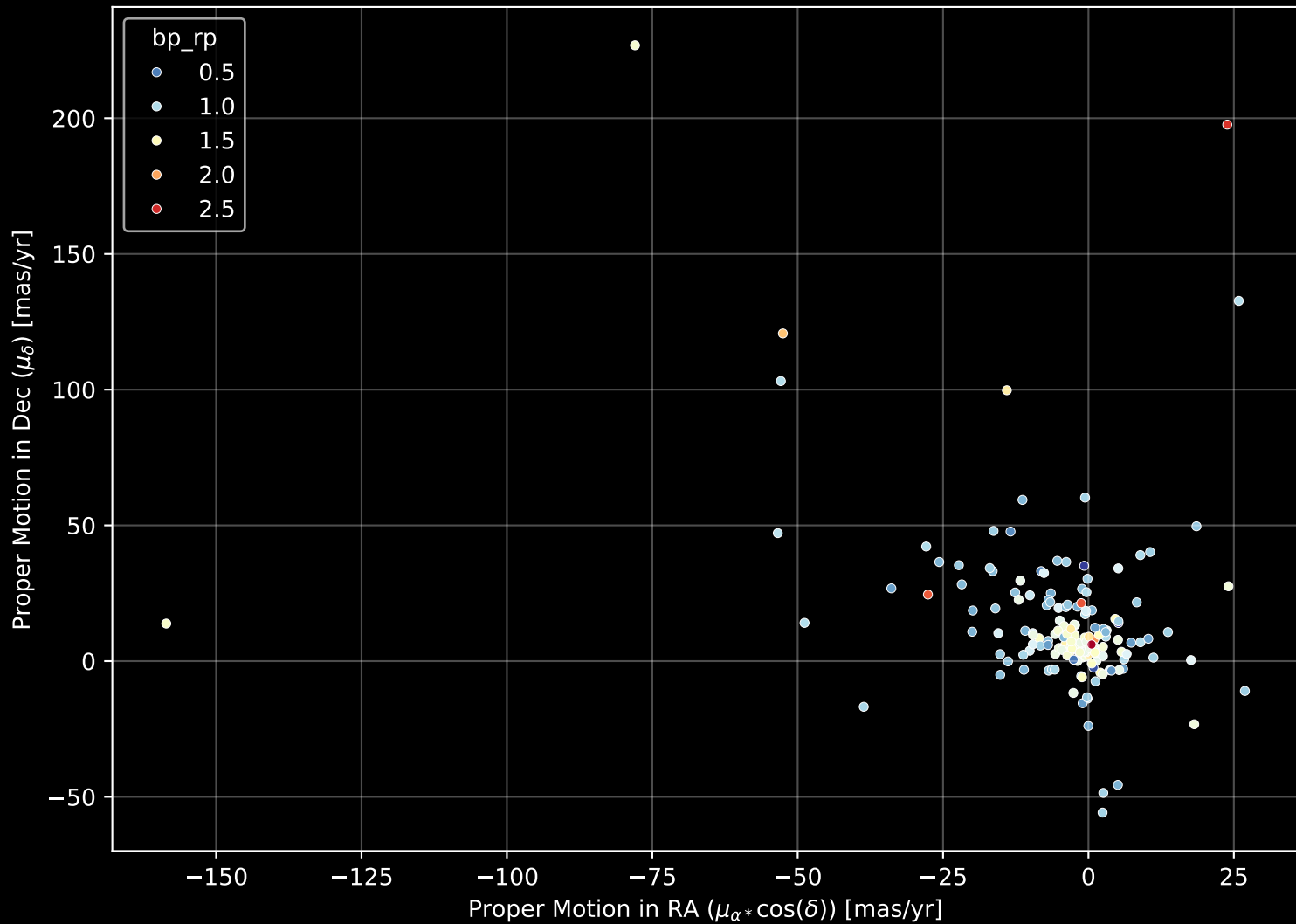
APOGEE DR17 Field: [279-24-O_TESS] Proper Motion Diagram (n= 168)
